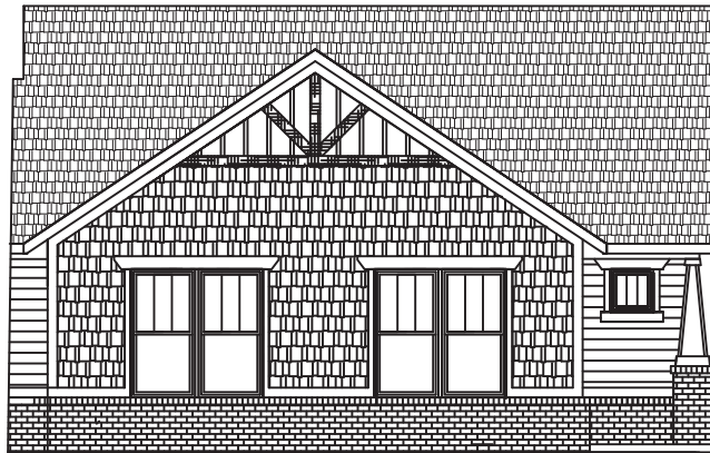
CRAFTSMAN FRONT ELEVATION
